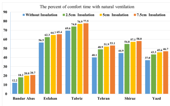
Figure 4. The percent of comfort hours in spring and summer for insulated and non-insulated sample building
