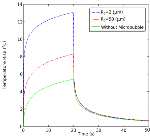
Figure 3. Temperature increase of biological tissue with respect to time for 20 seconds of irradiation and 30 seconds of the cooling process at the focal point in working conditions of 3 MHz and 1 W.
