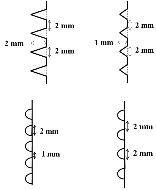
Figure 1. Triangular and circular grooves dimensions
