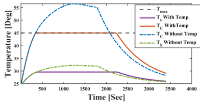
Figure 2. The Temperature evolution during fast charge with and without temperature constraint
