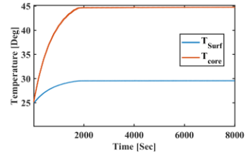
Figure 3. The temperature management of the cell under square wave current profile
