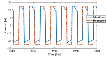
Figure 4. Restricting the applied current to manage the core temperature
