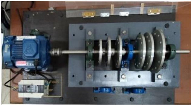
Fig. 1. Laboratory rotating machine for data recording
