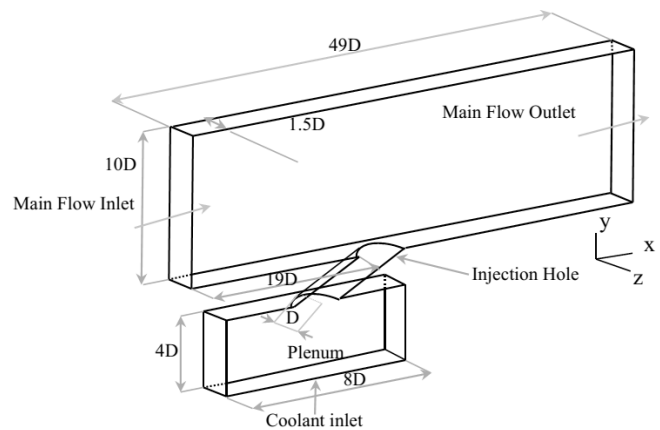
Fig. 1. Computational sketch based on the experimental work of Sinha et al. [1].
