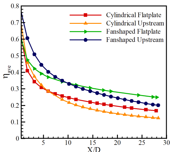
Fig. 2. The laterally averaged film cooling effectiveness for M=0.5
