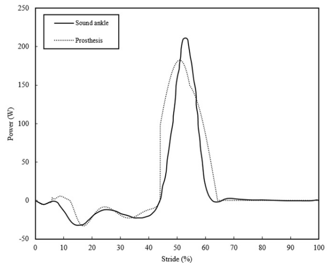
Fig. 4. Ankle power during one stride for the proposed prosthesis in comparison with the natural ankle data in [8].
