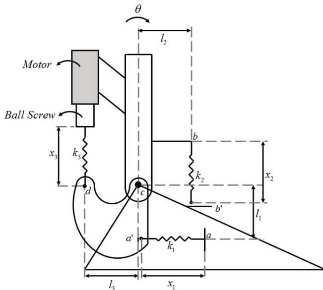
Fig. 1: Schematics of the proposed prosthesis
