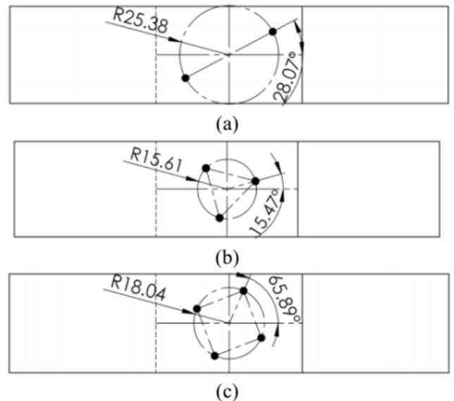
Fig. 6. Optimal location (a) 2 spots welding (b) 3 spots welding (c) 4 spots welding
