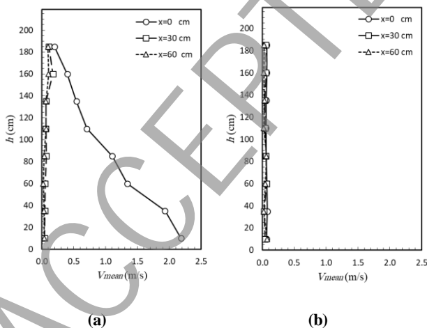
Fig 3. Velocity distribution for (a) vertical and (b) horizontal supply air diffuser
