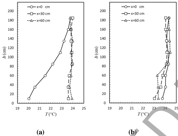
Fig 2. Temperature distribution for (a) vertical and (b) horizontal supply air diffuser
