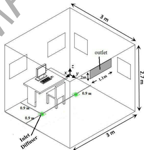
Fig 1. Climate chamber geometry
