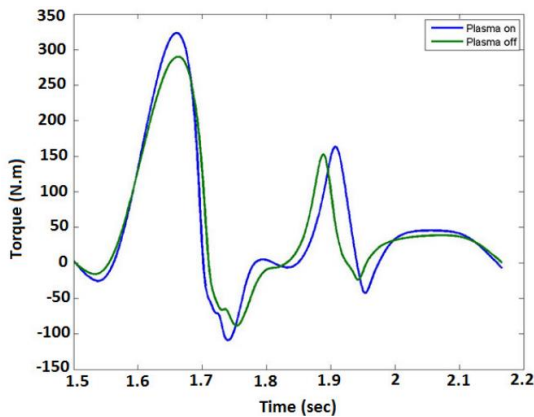
Figure 2. Torque variation vs. time with and without plasma actuator
