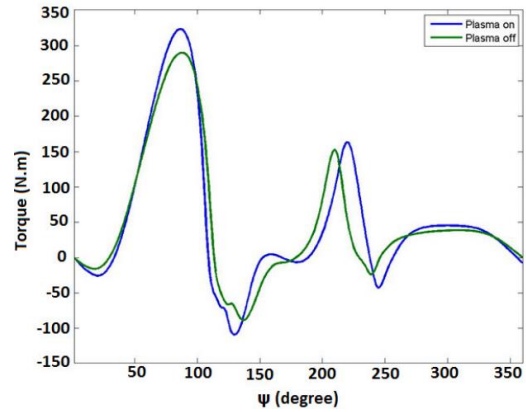
Figure 3. Torque variation vs. azimuthal angle with and without plasma actuator
