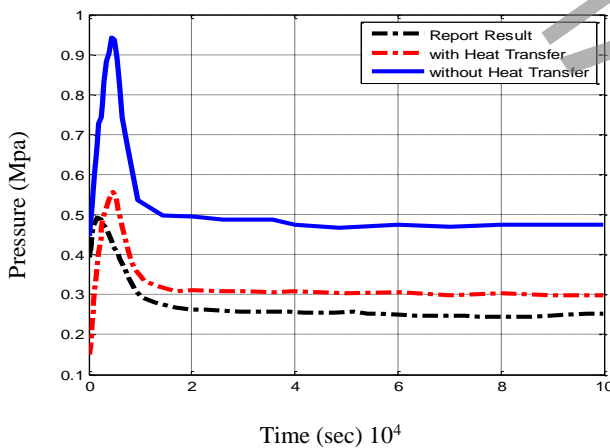
Fig.4. Time variations of safety containment Pressure
