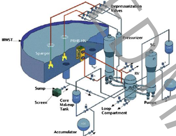
Fig.1. AP1000 RCS and Passive Core Cooling System [1].
