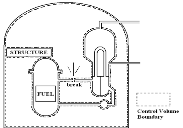
Fig. 2. Control Volume
