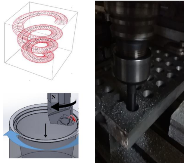
Figure 1. Schematic and actual views of thread milling
