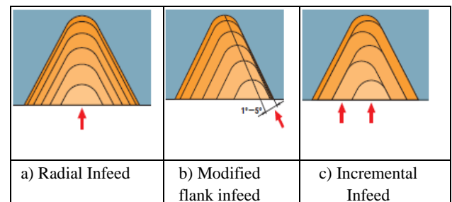
Figure 2. Infeed methods in thread cutting.
