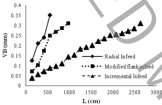
Figure 4. Dependence of the tool wear to the length of cutting, using N=700 rpm and f=0.4 mm/rev.
