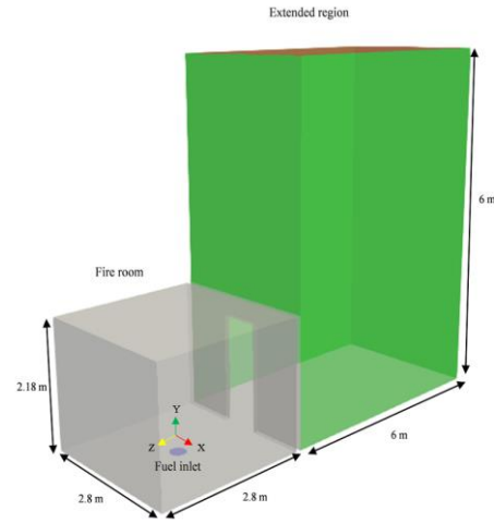
Figure 1. Geometry of the one-room compartment in the current study
