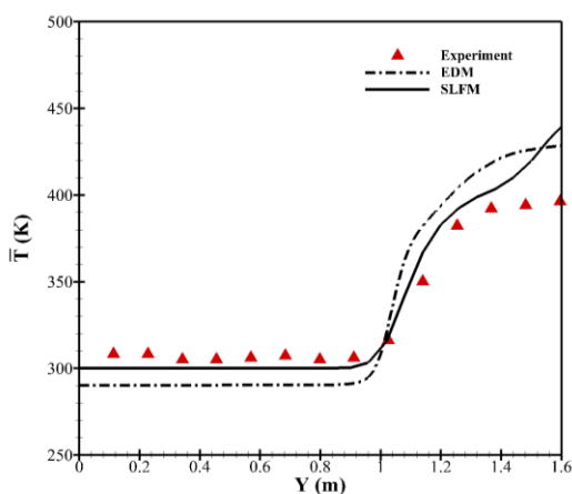
Figure 3. Comparison of numerical and experimental results for the average temperature at the doorway
