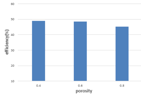
Figure 5. Comparison of radiation efficiency for different porosity
