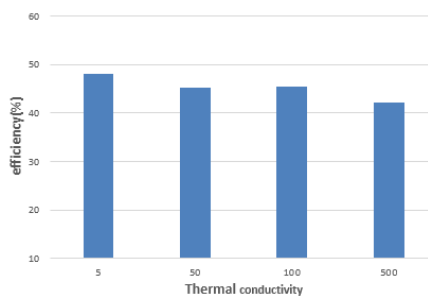
Figure 4. Comparison of radiation efficiency for different thermal conductivity of porous
