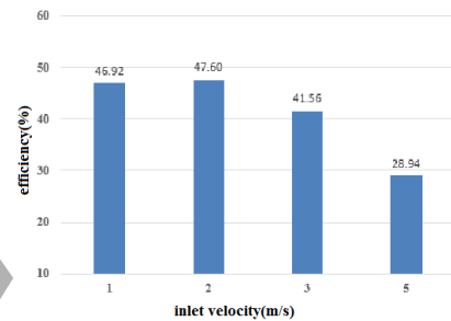
Figure 6. Comparison of radiation efficiency for different inlet velocity
