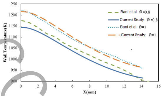
Figure 2. A Comparison of wall temperature results in the present study with the reference [9].
