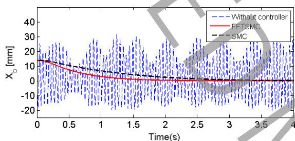
Figure 7- Simulation results of the feedback system under the fuzzy fast terminal SMC
