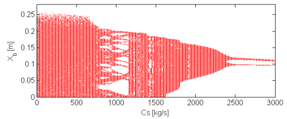
Figure 3- Bifurcation diagrams of X_b with relative to equal damping coefficient of the active suspension system
