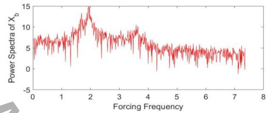
Figure 4- Power spectrum density diagram of the displacement in the body of vehicle
