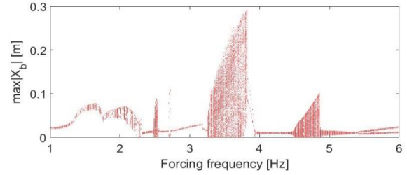
Figure 2- Bifurcation diagrams of X_b with relative to Frequency of the excited force from road surface
