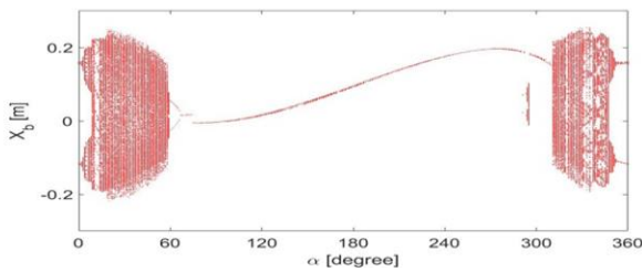
Figure 1- Bifurcation diagrams of X_b relative to \alpha
