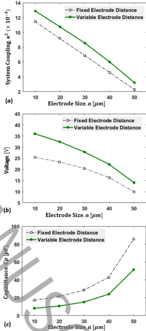
Figure 2: Nanogenerator's performance versus the electrode size for open circuit condition and L_E(1) = 60 micron, (a) system coupling, (b) Maximum output voltage, (c) nanogenerator's capacitance
