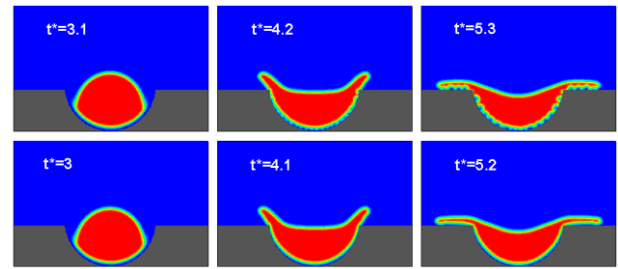
Figure 3 Results obtained for sequence of droplet collision into a semicircular cavity with density ratio 1000, viscosity ratio 100, Re = 80 and Bo = 5000 at contact angle of 40 (top row) and 170 (bottom row).
