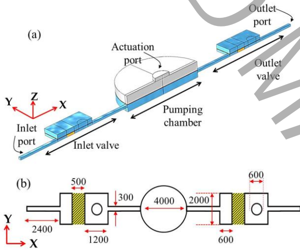
Figure 1. (a) Three dimensional design, and (b) Schematic design of micropump, dimensions are in microns.
