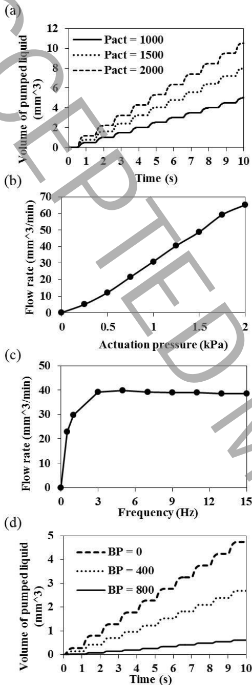
Figure 3. (a) Time-domain pumped liquid volume, (b) Flow rate of micropump versus actuation pressure, (c) Flow rate of micropump versus actuation frequency, (d) Time-domain pumped liquid volume with different backpressure at micropump's outlet.
