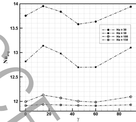
Fig. 14. Variations in the Nusselt number according to the magnetic field applying angle and Ra=1E5 , Da=5E-5 , k_{eff}=10
