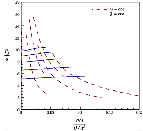
Fig. 4. Variations of the dimensionless radius versus the dimensionless swirl number
