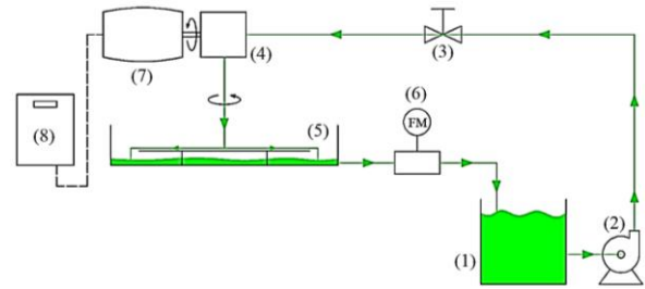
Fig. 2. The schematic of the device designed and built to create hydraulic jumps of the present study; 1) major fluid storage tank, 2) pump, 3) flow control valve, 4) gearbox, 5) overflow tank and target plate, 6) flow meter, 7) electric motor and 8) regulating device of fluid jet swirl velocity.
