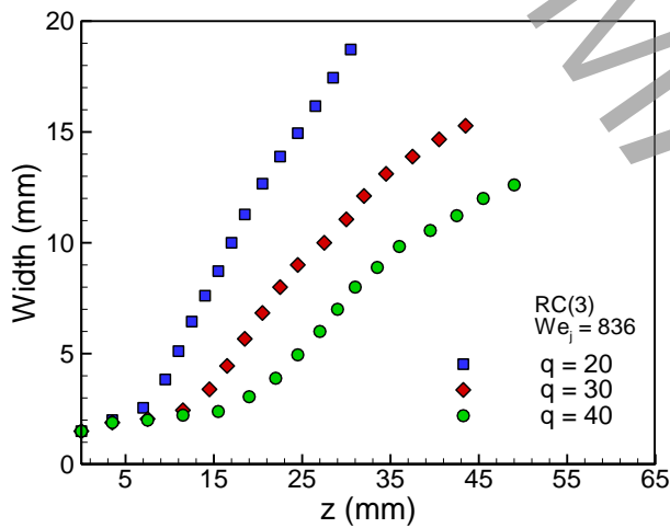
Figure 2. Variation of RC(3) jet width at different momentum ratios for constant jet Weber number of 836.
