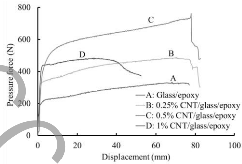
Figure 3. Effect of adding CNTs with different weight percentages on the force-displacement graph of composite plates
