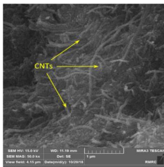
Figure 4. Homogeneous dispersion of CNTs into the matrix material for 0.5% CNT/glass/epoxy composite plate
