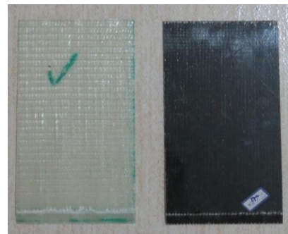
Figure 1. Glass/epoxy composite plate sample (left) and CNT/glass/epoxy composite plate (right)
