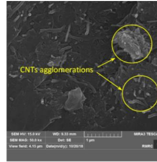
Figure 5. Nonhomogeneous Dispersion of CNTs into the matrix material for 1% CNT/glass/epoxy composite plate and existence of CNTs agglomerations
