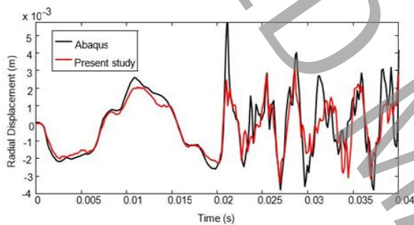
Figure 1. Comparison of time response (radial displacement) in the middle of the cylinder
