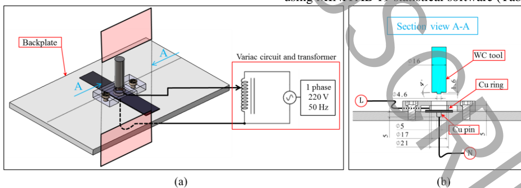
Figure 1. (a) Schema of the electrically-assisted equipment and (b) longitude section with dimensions (mm)
