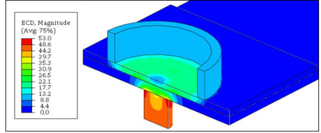
Figure 2. Current density distribution at 500 A
