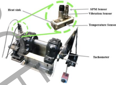
Figure. 4. The test-rig for the REB accelerated-life test
