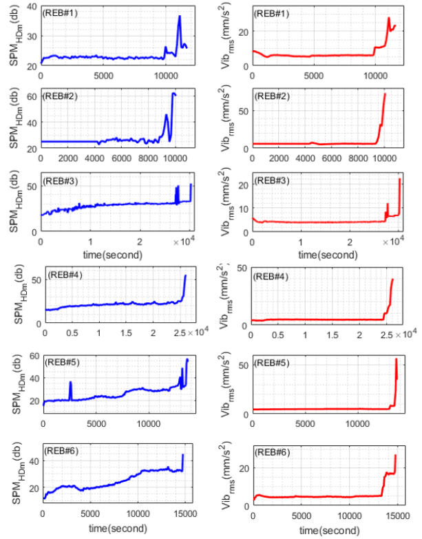
Figure. 5. The comparison between the trend of SPM_{HDm} and V_{rms} for all six accelerated-life experiments
