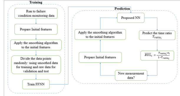
Figure 1. The proposed algorithm for RUL prediction of REBs
