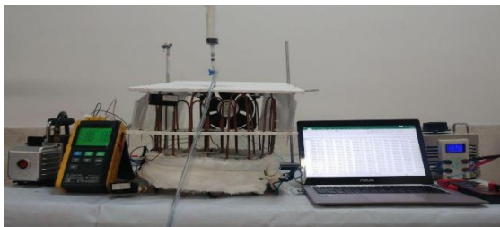
Figure 1. Testing system and its related equipment
