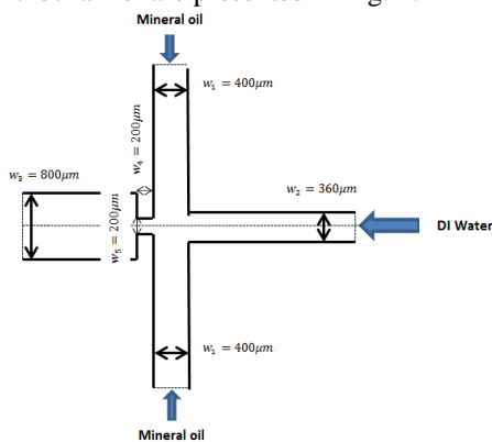
Figure 1. Dimensions of the microchannel built to control the size of generated droplets
