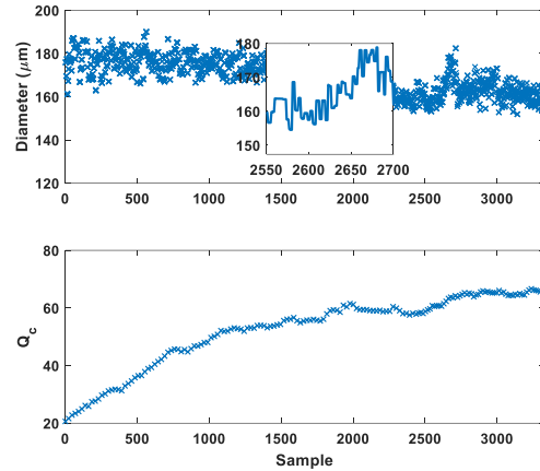
Figure 4. The effect of the disturbance and the response of the controller (RSME = 0.48).
