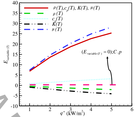
Fig. 2. Variations of the average heat transfer coefficient of the base fluid for variable properties to constant properties at different heat fluxes for Re=1000.
