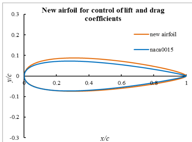
Fig.4. New airfoil at AOA=8^\circ
