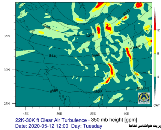
Fig. 3. Prediction of clear air turbulence for 22K-30K ft level at 12 UTC on May 12, 2020.
