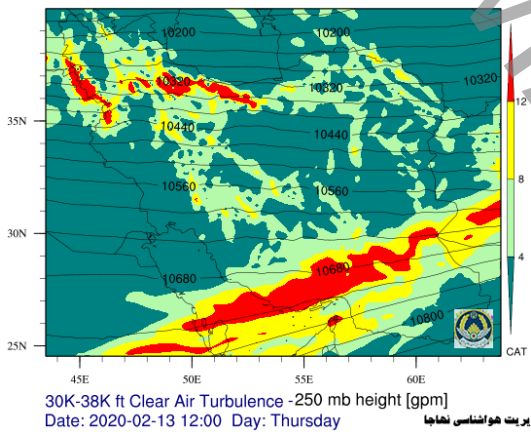
Fig. 2. Prediction of clear air turbulence for 30K-38K ft level at 12 UTC on February 13, 2020.
