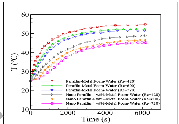
Fig. 3. The effect of Reynolds number of pure water flow in a combined system the pure water as working fluid and two cases in the passive part, including paraffin-metal foam and 4% nano-paraffin-metal foam in the cooling system at (a) 4.5 Watts and (b) 14 Watts
