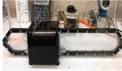
Figure 1. Set up of thermal management system with plate heater
