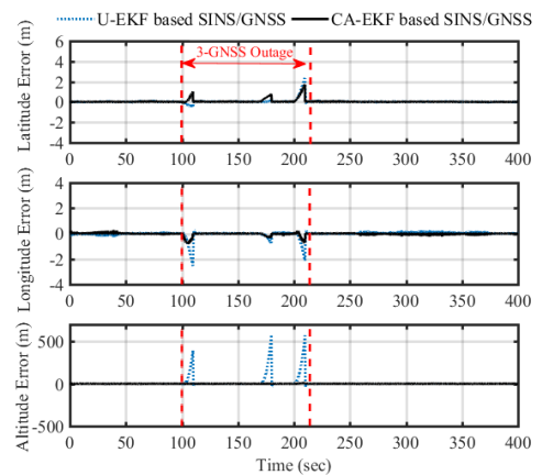
Fig. 5. Estimation error of vehicular positions
