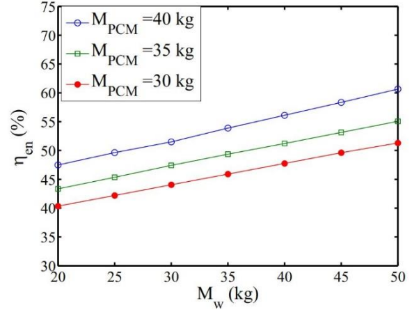
Fig. 2. Average daily energy efficiency based on changes in PCM and water masses
