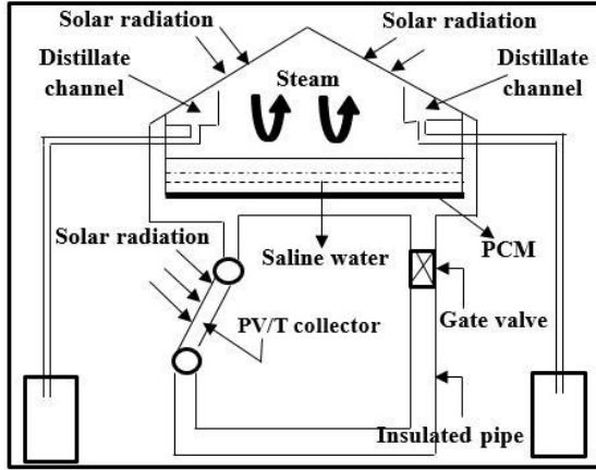
Fig. 1. Double slope basin solar still equipped with PCM and PV/T collector
