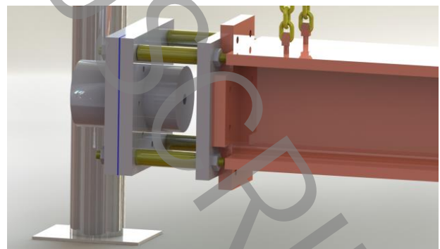
Figure 1. Ballistic pendulum
