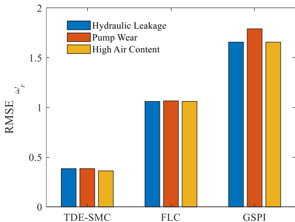
Fig. 1 RMSE of rotor speed in the presence of different faults
