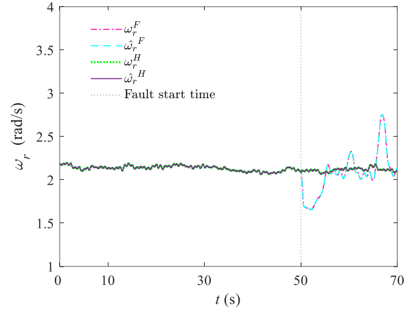
Fig. 2 rotor speed for both healthy and faulty conditions
