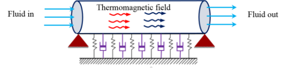
Figure 1. Schematic of single-walled CNT conveying fluid
