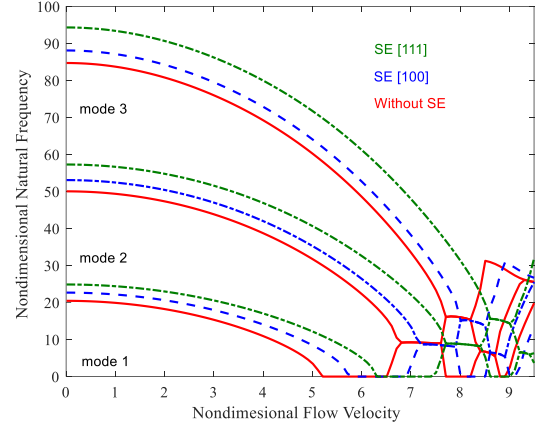
Fig. 3. The surface effect on the non-dimensional frequency at mode 1 to 3 of single-walled CNT conveying fluid with C-C boundary condition
