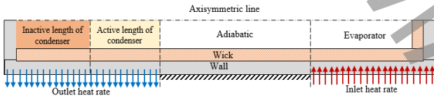
Figure 1. Schematic of variable conductance heat pipe
