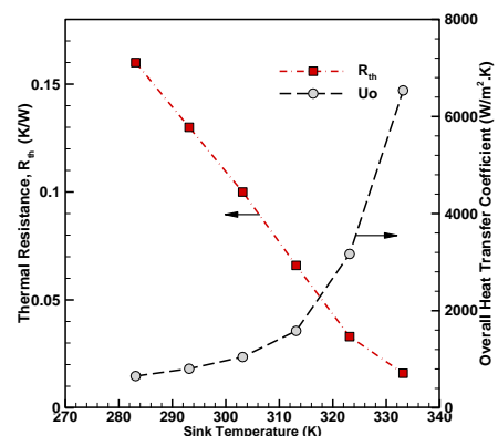
Figure 3- Changes in thermal resistance and overall heat transfer coefficient versus the sink temperature
