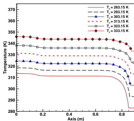
Figure 2- Effect of sink temperature on wall temperature profile
