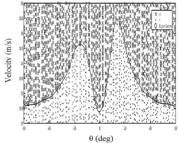
Fig. 2. Training support vector machine with 2100 samples
