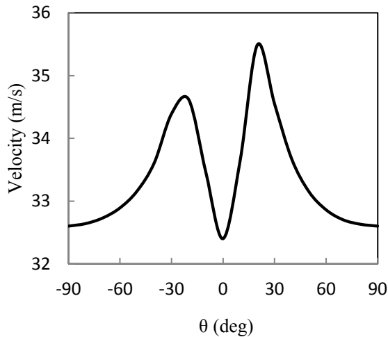
Fig. 1. Flutter speed of composite wing against fiber orientation
