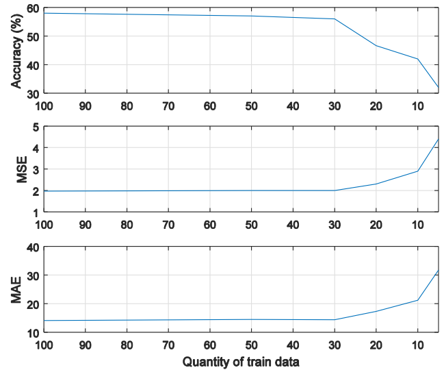
Fig. 2. Comparison of prognosis measures for different sizes of train data
