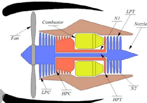
Fig. 1. Simplified diagram of the gas turbine engine [3]
