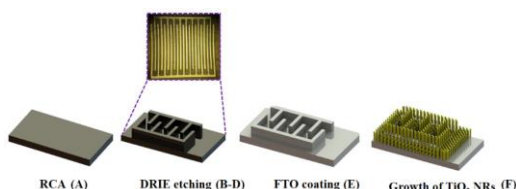
Figure 1. Graphical schematic of the manufacturing process of FTO / TiO 2 NRs and the real etched sample
