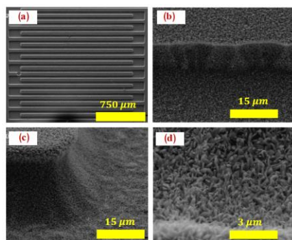
Figure 3: SEM images of TiO 2 nanowires on micromachined silicon substrate
