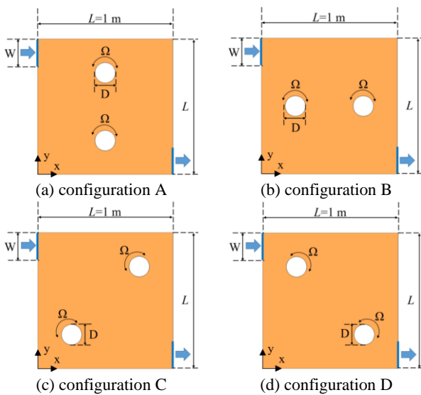
Figure 1. Schematic view of the computational domain.
