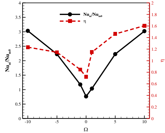
Figure 3. Ratio of average Nusselt number on the bottom wall of cavity and performance evaluation criteria for different rotational velocity of rotating cylinders for configuration D ( \phi_{hnf}=0.03 , Re=250 )
