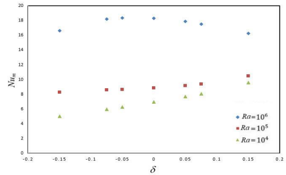
Figure 3. Variations of the average Nusselt number of the heat source surface for the flexible system for different values of Ra and \delta
