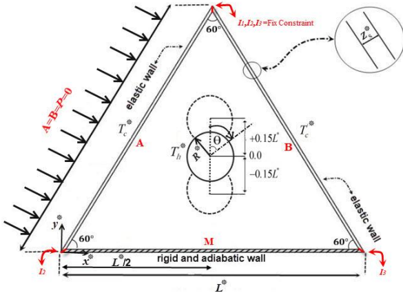
Figure 1. Geometry of the present study
