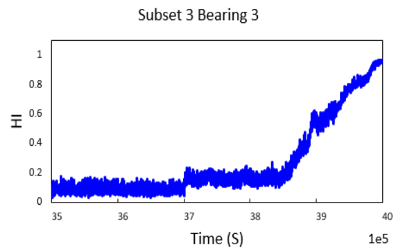
Figure 2. Bearing health indicator during failure stage.
