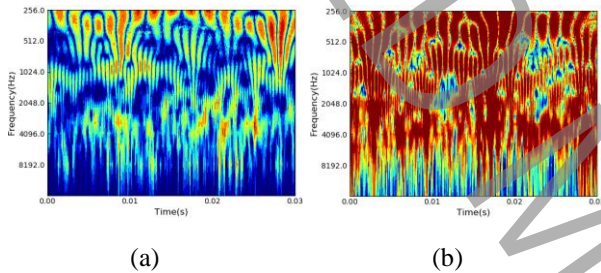
Figure 1. (a) CWT image of healthy stage, (b) CWT image of failure stage.
