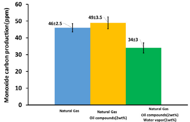
Fig. 5. Effect of nebulizer injection of various compounds on CO emissions
