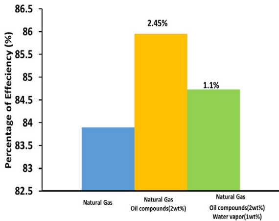
Fig. 2. Effect of nebulizer injection of various compounds on thermal efficiency
