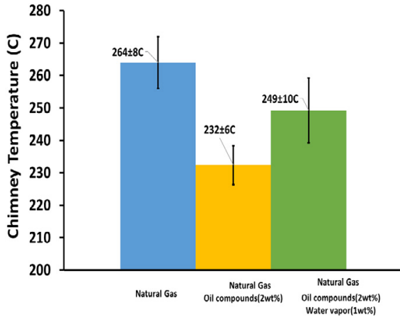
Fig. 1. Effect of nebulizer injection of various compounds on the chimney outlet temperature
