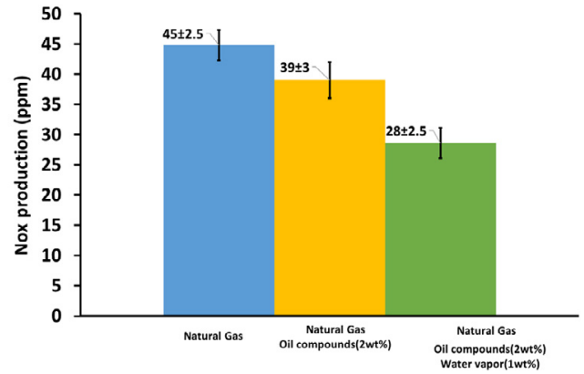
Fig. 4. Effect of nebulizer injection of various compounds on NOx emissions
