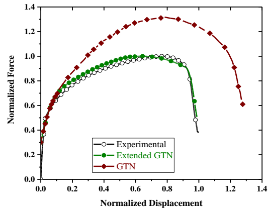
Figure 1. Experimental and numerical force-displacement curves for shear specimen
