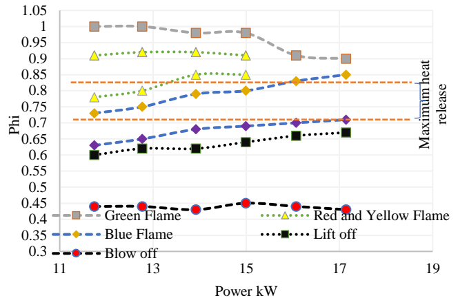
Fig 5- functional diagram for operating burner power versus equivalence ratio
