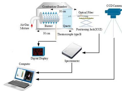
Fig 2- Schematic of the combustion chamber, CCD camera, and spectrometer
