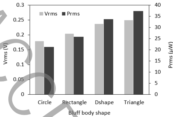
Fig. 1: effect of the bluff body shape on the harvester performance
