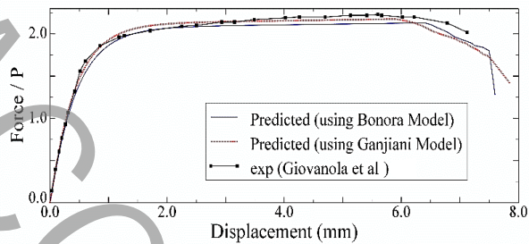
Figure 1: The comparison of force-displacement between simulation and the result of ref. [52] for steel HY130.
