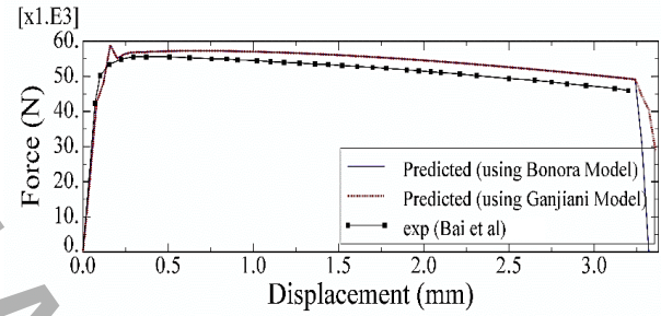
Figure 1: The comparison of force-displacement between simulation and the result of ref. [34] for steel 1045.
