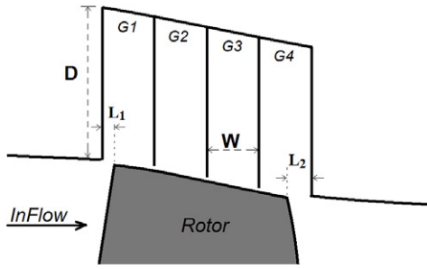
Fig. 1. Casing treatment configuration
