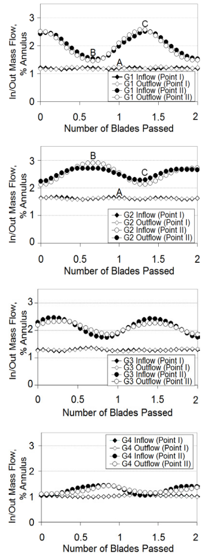
Fig. 3. Time histories of the mass flow rate into and out from each groove.
