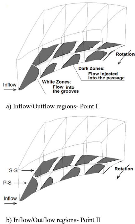
Fig. 4. Time-averaged inflow/outflow regions
