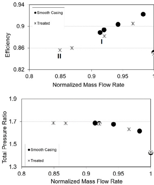
Fig. 2. Compressor characteristic
