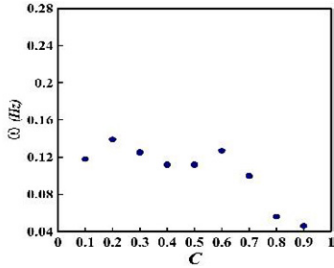
Fig. 2. The average value of the frequency of Holmboe waves at different densities of intrusive gravity current
